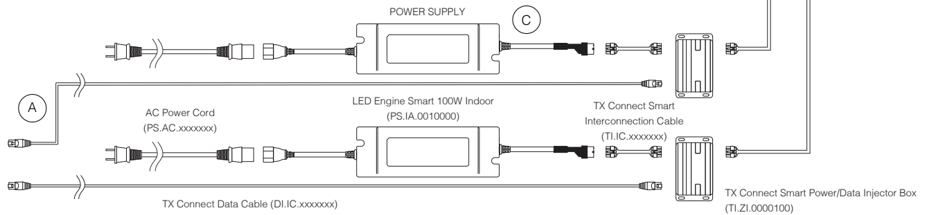
CONTROLLER Powered by LED Engine via TX Connect Data Cable
